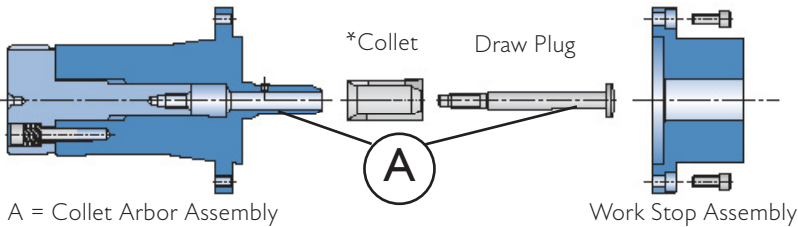
3J Collet-Style, #200, 250 and 300
