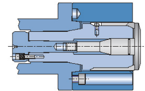
16C Collet-Style
