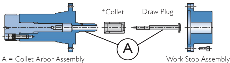
16C Collet-Style, #200, 250 and 300
