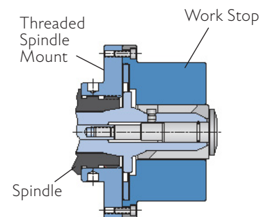
#400, #500 5C Collet-Style
